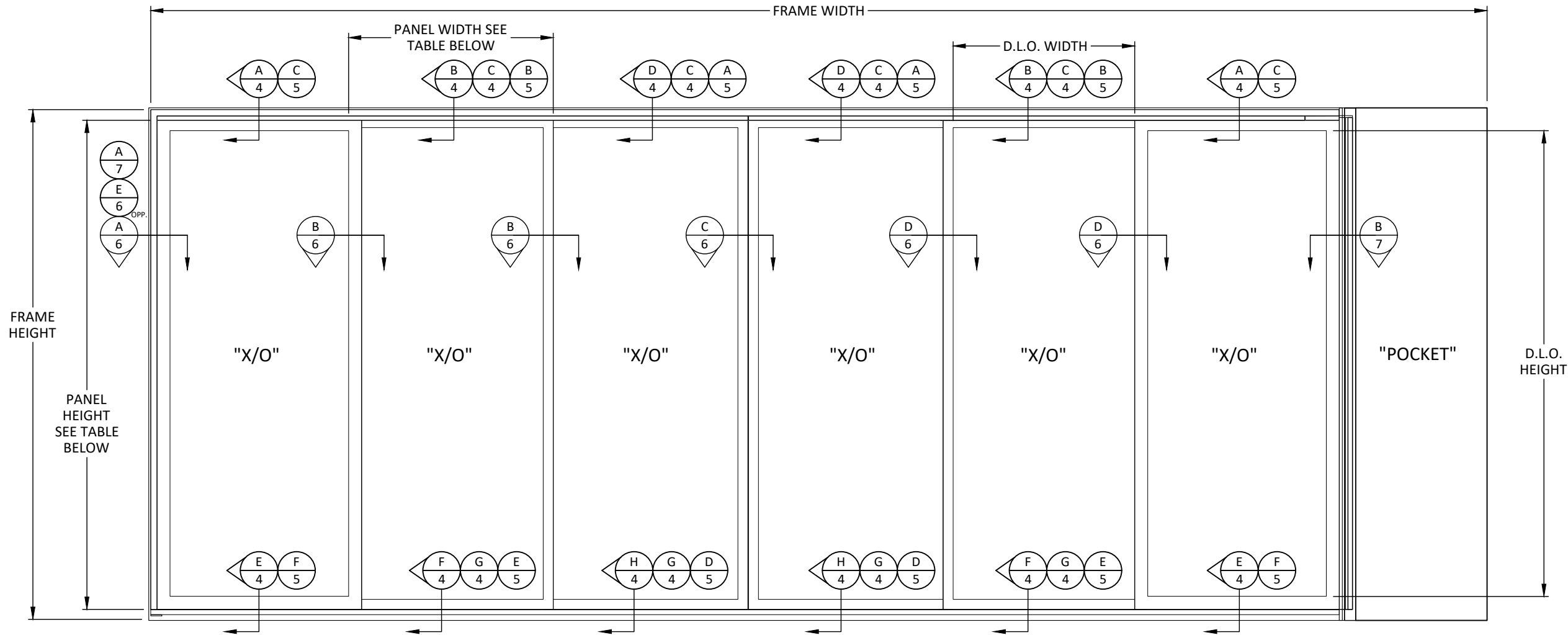
TYPICAL ELEVATION LIFT & SLIDE DOOR
