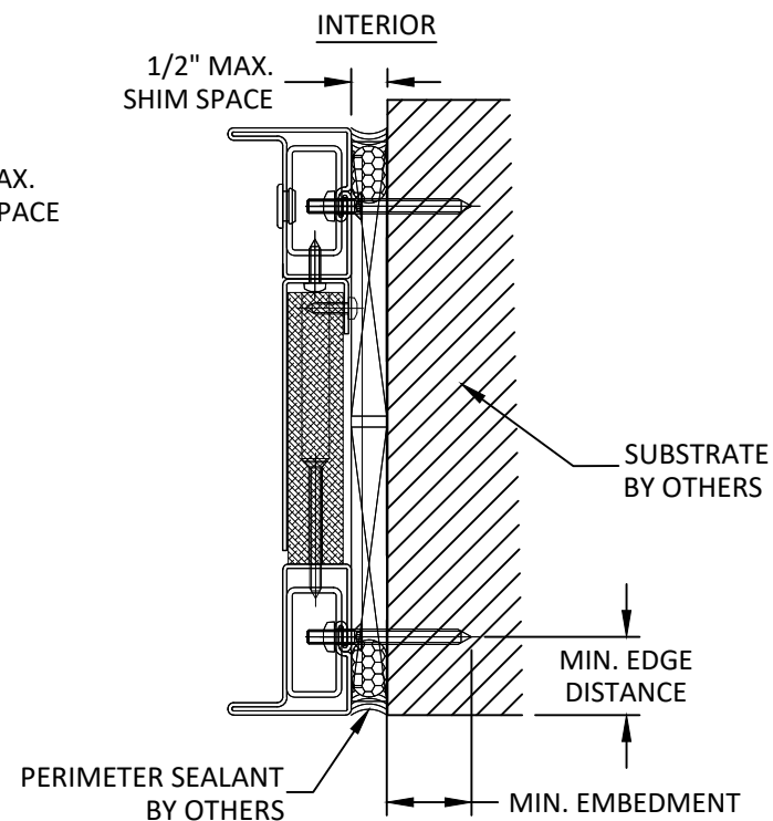
C 8 INSTALLATION DETAIL THROUGH FRAME 2-TRACK JAMB
