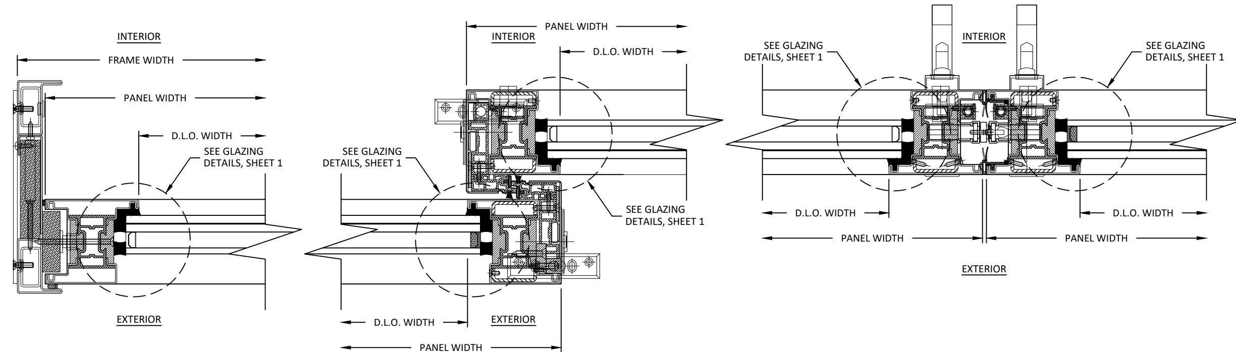
A 6 HORIZONTAL SECTION 2-TRACK JAMB FIXED PANEL - OUTSIDE GLAZED
