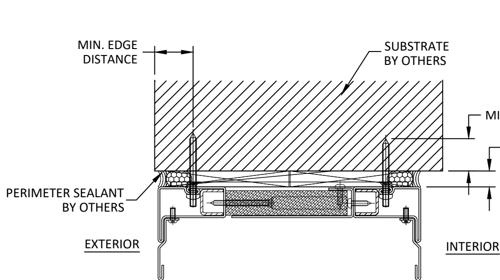
A 8 INSTALLATION DETAIL THROUGH FRAME 2-TRACK HEAD
